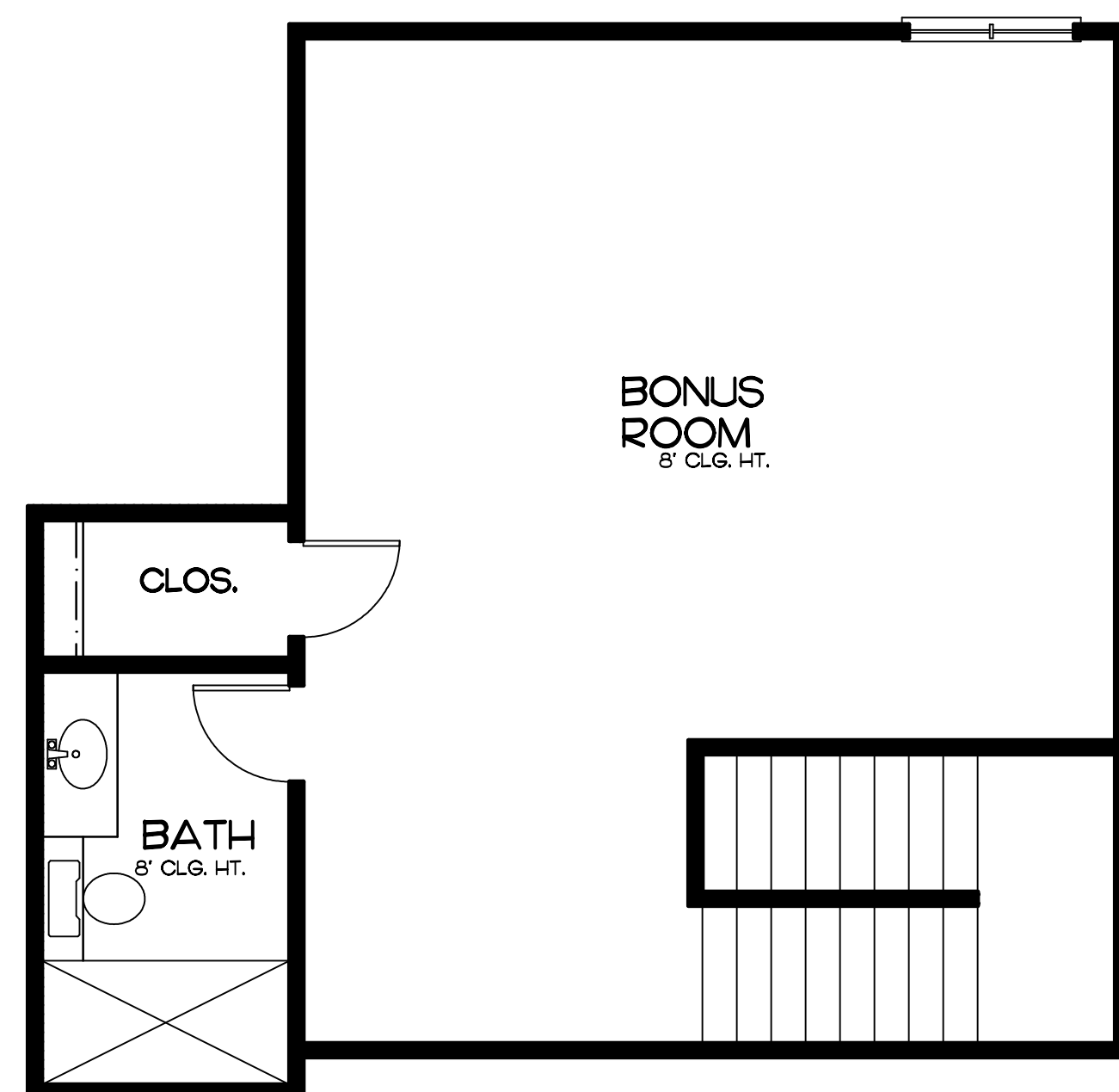
UPPER FLOOR
