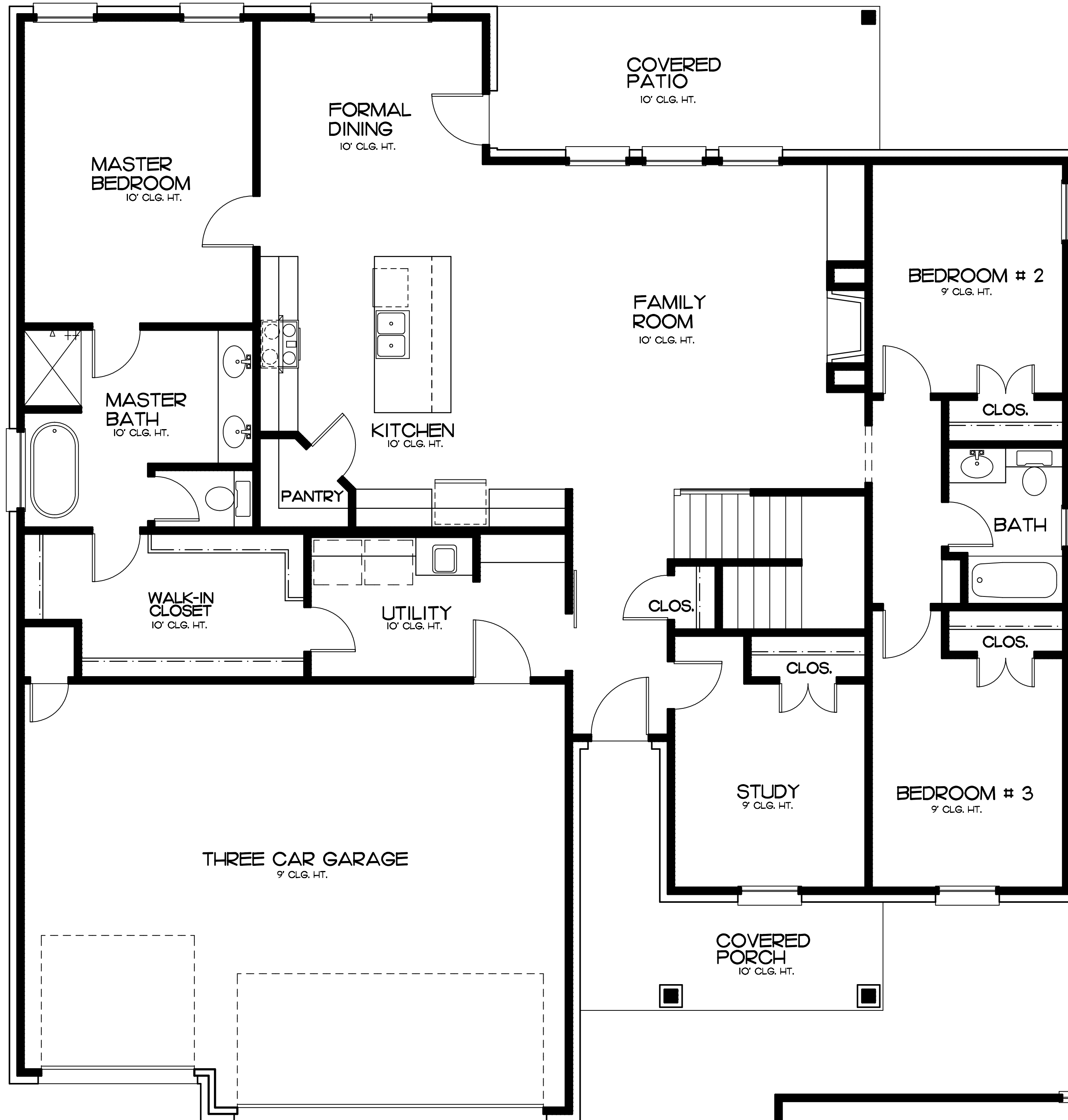
LOWER FLOOR
