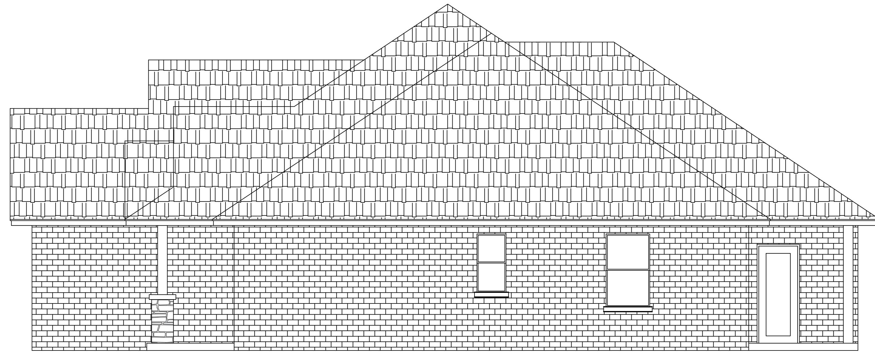
LEFT ELEVATION 1/4" = 1'-0"
